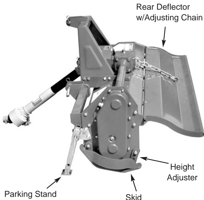
Figure 3-1 Adjustments
